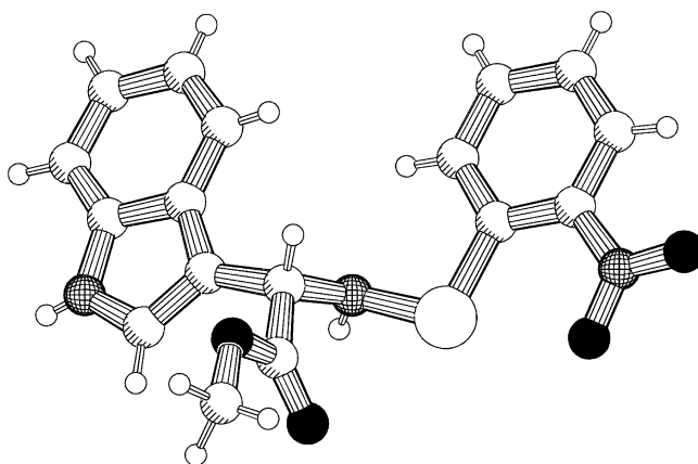
Figure 1. X-ray structure of ( S )- 3 .
